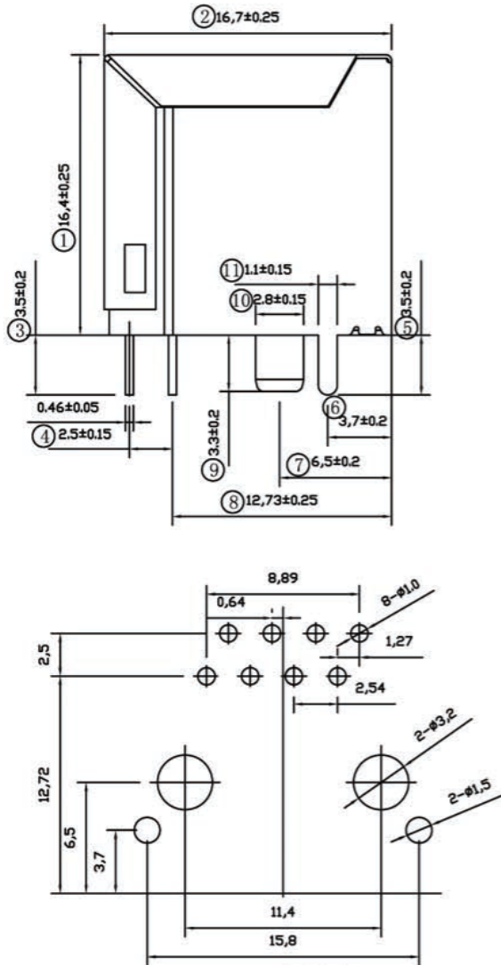
P.C.B Reference drawing
