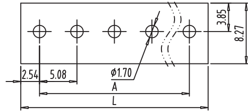
PCB LAYOUT S=2:1
