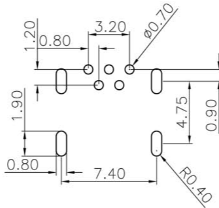
PCB LAYOUT
