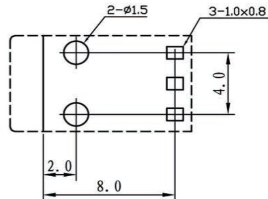
Schematic of PCB Installation Dimensions
