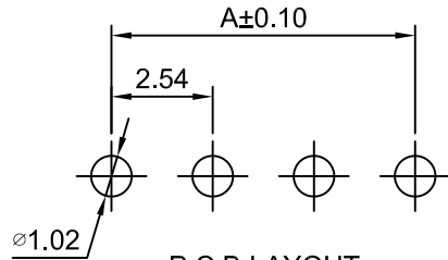
P.C.B LAYOUT TOLERANCE:±0.05
