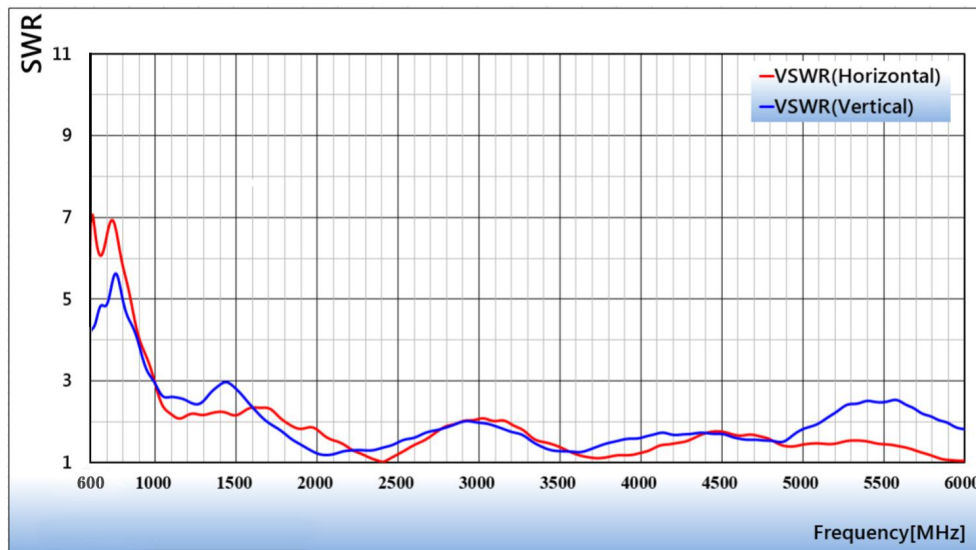
Graph1. KH6G-0H-08 VSWR
