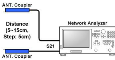
Figure2. Test Setup
