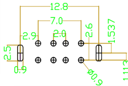
RECOMMENDED P.C.B PATTERN LAY OUT
