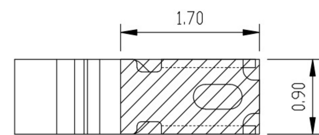
Welding Chassis Dimensions
