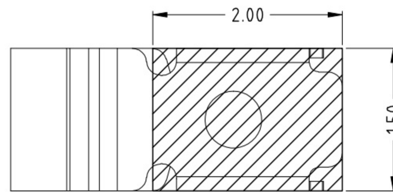
Welding Chassis Dimensions Dimensional Tolerances ± 0.05
