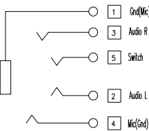
SCHEMATIC(PLUG OUT)
